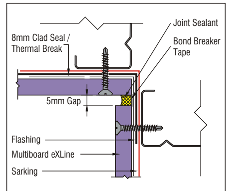
Figure 20 - Internal Sealant Fill Corner Detail
