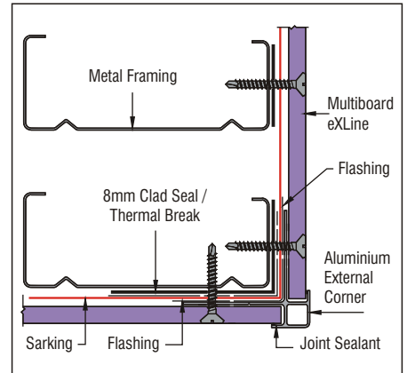
Figure 18 - External Aluminium Corner Detail
