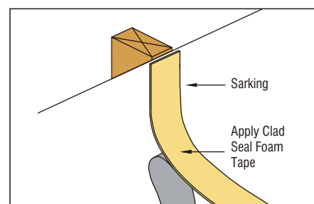
Figure 1 - Apply Clad Seal Foam Tape at Joint Locations
